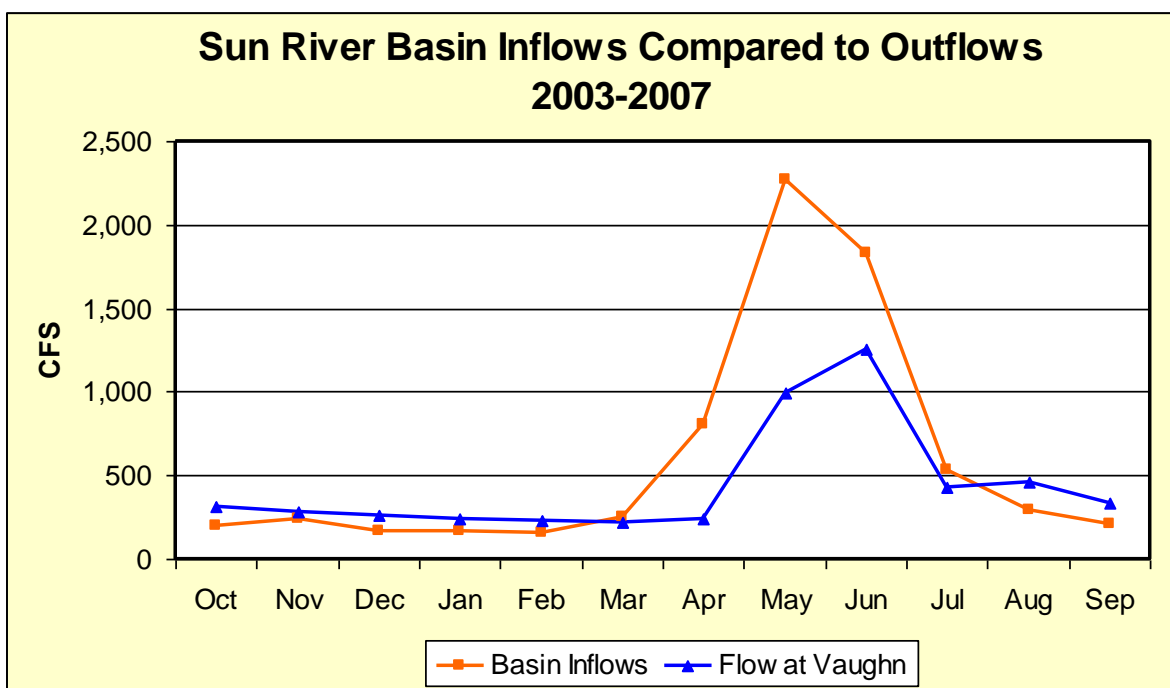
Figure 2. Sun River Basin inflow/outflow comparison.
